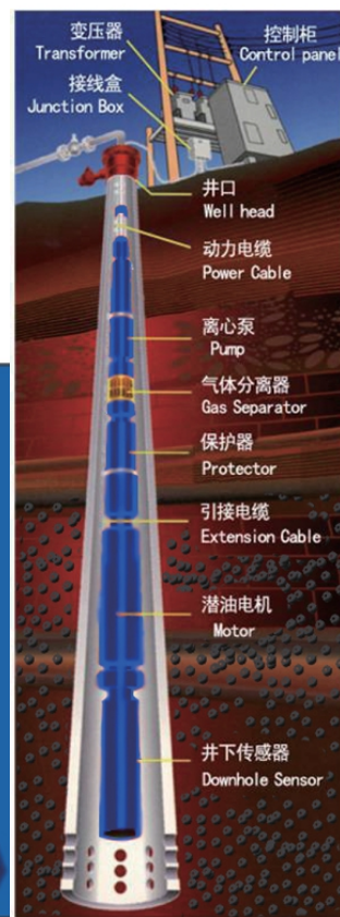
electrical submersible pump (ESP)
