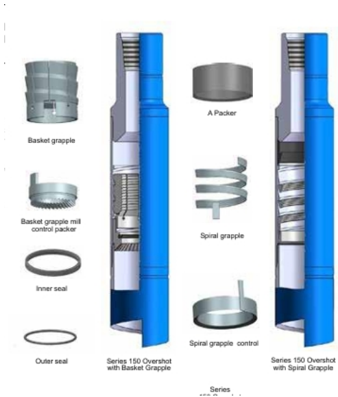
Releasing and Circulating Overshot
