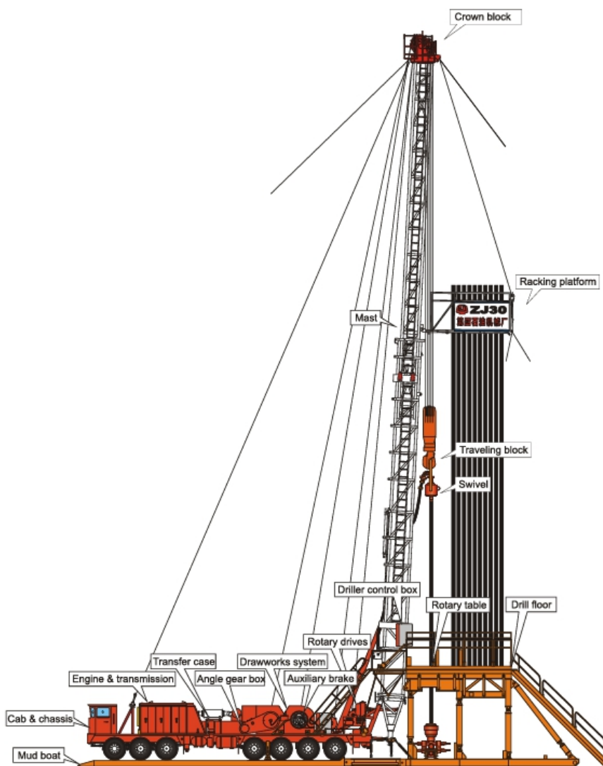
3000m Truck-mounted drilling rig
